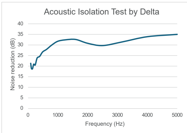
Typical damping effect of Miljøskærm noise barrier element
